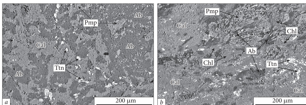
Fig. 13. Fine-crystalline (a) and needle-shaped (b) segregations of pumpellyite in metabasalt. BSE image
