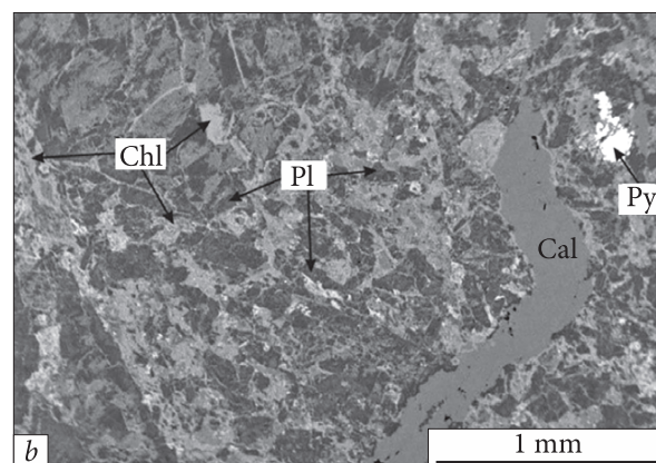
Fig. 8. Development of chlorite in metabasalts, BSE image. Minerals: Pl — plagioclase, Py — pyrite (see Fig. 7 for the rest)
