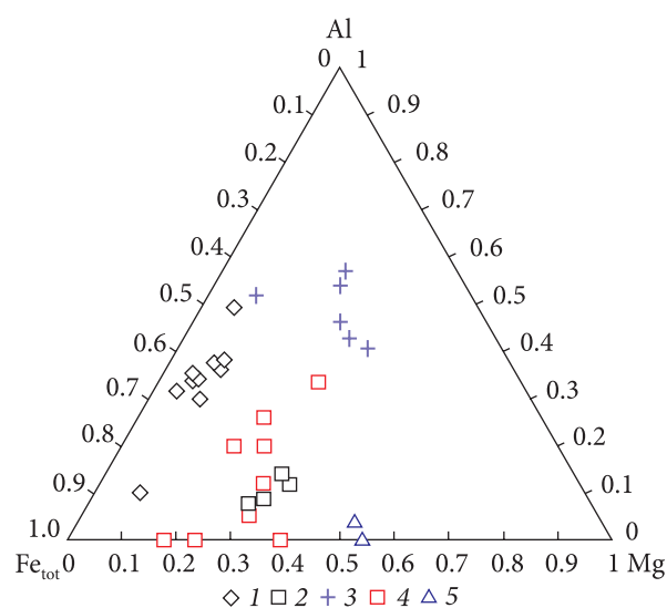
Fig. 14. Variations in the composition of pumpellyite from various rocks in the three-component system \text{Fe}_{\text{tot}} -Al-Mg (formula coefficients), according to [25] with authors additions: 1 — metabasalts of the Uholskyi complex; 2 — metabasalts of the Rakhivsko-Chyvyhynskyi complex; 3 — metadiabases [25]; 4 — volcanic-sedimentary metabasites [18]; 5 — effusive rocks of the basic composition [10]
