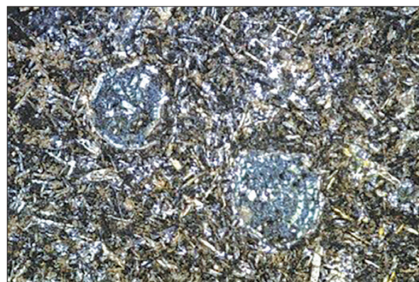
Fig. 12. Chloritized and carbonatized metabasalt of the Uholskyi complex; field of view — 2 mm, XPL
