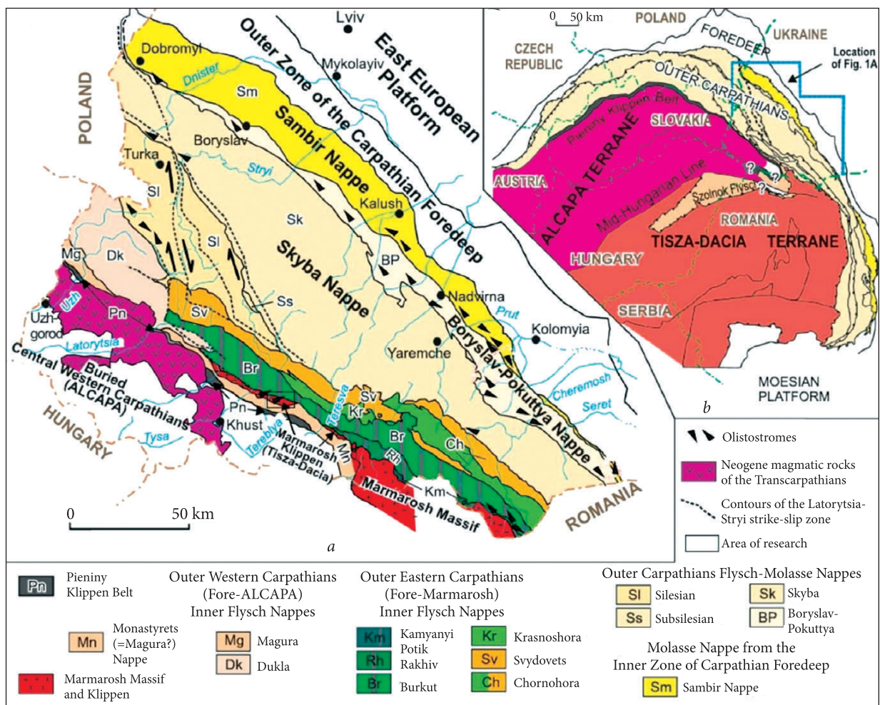
Fig. 1. Main tectonic units (a) and tectonic position of the Ukrainian Carpathians (b) according to O. Hnylko [9]
