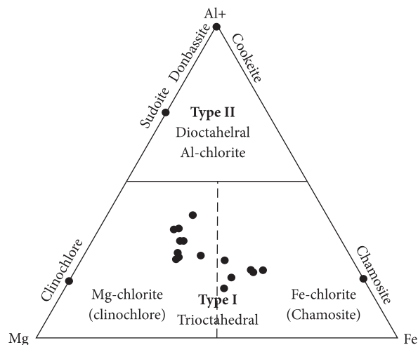
Fig. 9. Classification diagram of the compositional fields of rock-forming chlorites according to [28]
