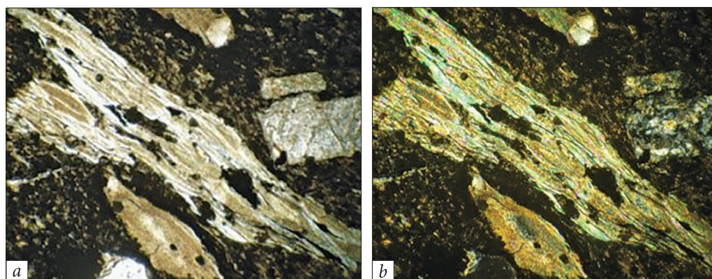
Fig. 6. A lens of secondary minerals (muscovite, carbonates, etc.) in metabasalts, field of view — 2 mm: a — PPL; b — XPL
