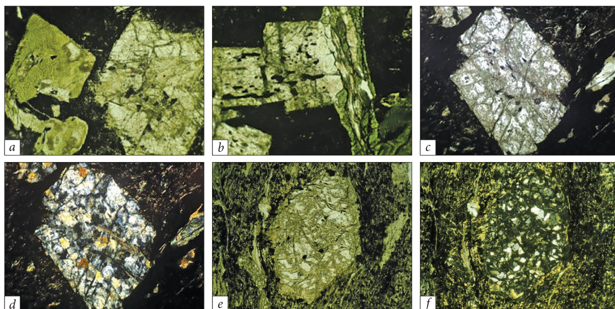
Fig. 5. Phenocrysts of altered plagioclase from metabasalts, field of view — 2 mm: a, b, c, e — PPL; d, f — XPL. Secondary minerals: a, b — chlorite, pumpellyite; c, d — pumpellyite, quartz; e, f — chlorite, pumpellyite, quartz
