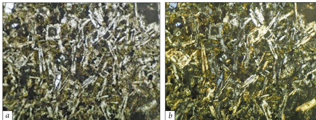
Fig. 4. Spilitic texture of metabasalts, field of view — 2 mm: a — plane-polarised light (PPL); b — cross-polarised light (XPL)
