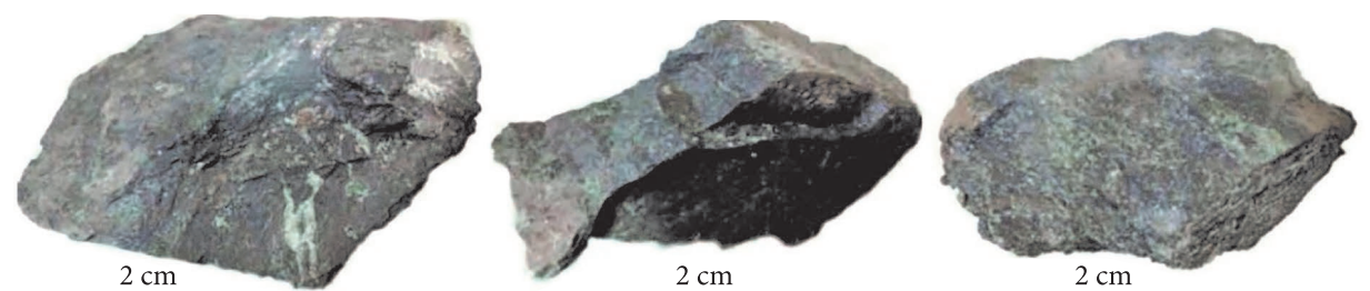
Fig. 3. Metabasalts of the Rakhivsko-Chyvchynskyi complex (Kamianyi Potik)
