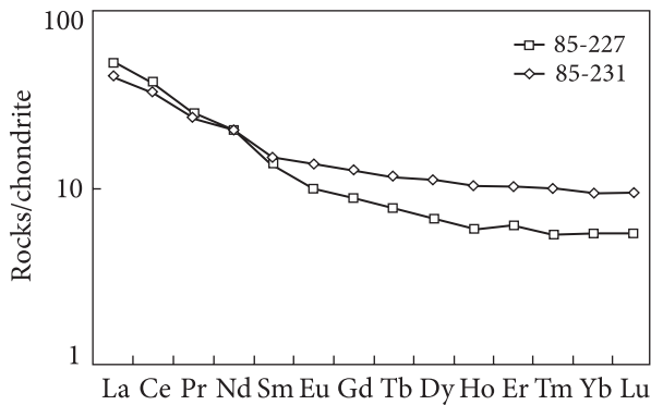
Fig. 3. Chondrite-normalized REE pattern for the quartz-amphibole schists for the sedimentary-volcanogenic rocks of the Chortomlyk iron deposit. Chondrite composition after (Sun, McDonough, 1989)
