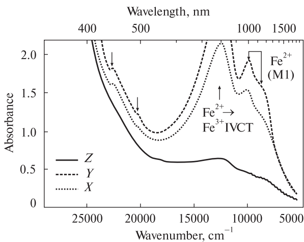
Fig. 4. Polarized absorption spectra of augite 741/278.5-1 from fenitized syenite
